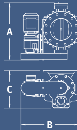
BSM Chain Drive
