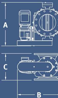
HDM Chain Drive
